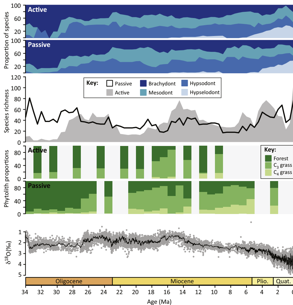
Figure 3. Climatic and Biotic Changes in North America over the Past 35 myr. The global temperature trend is from the benthic foraminiferal oxygen-isotope record (data from [76]). Notable warming during the Middle Miocene was followed by long-term cooling and Quaternary glacial cycles. Global climate influenced vegetation (inferred from the phytolith record) differently in the active (montane west) versus the passive (Great Plains) regions of North America (data from [77–80]). Although both regions exhibited a Neogene increase in grasses, the decline of forest ecosystems occurred earlier in the passive region. Between 34 and 28 Ma, 22 and 18 Ma, and 2 and 1 Ma, rodent diversity was higher in the passive than in the active region, whereas from 17 to 13 Ma, 7 to 5 Ma, and 5 to 3 Ma, diversity was much higher in the active region. The contrast in diversity between active and passive regions was greatest during the Miocene Climatic Optimum (17–14 Ma). Much of the diversity change among rodents coincided with changes in faunal composition [48,49]. Corresponding changes in dietary ecology are demonstrated by the increase in high-crowned species (hypsodont and hypselodont) toward the present day (data from J.X.S.). This increase preceded the expansion of grasslands in both regions, suggesting that adaptation to more abrasive diets was initially driven by volcanic ash in soils or grit on plants rather than increased consumption of grass.
